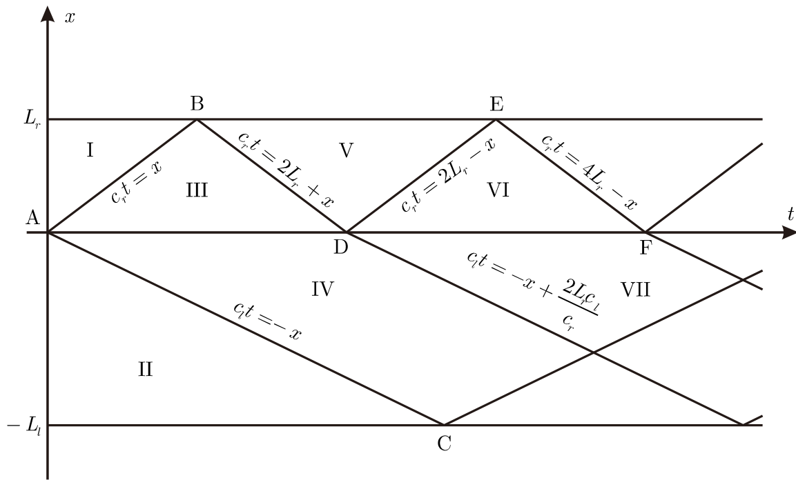
Figure 1: Space-time diagram
