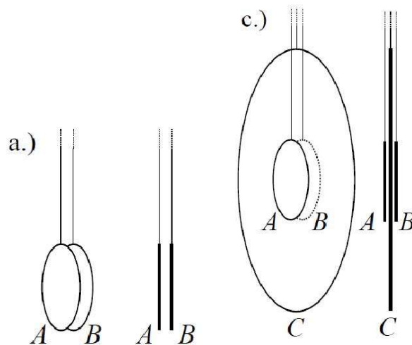
Figure 1: Charged discs set-up
